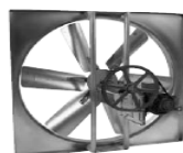
MODEL L Propeller Belt Drive Sidewall Exhaust or Supply
